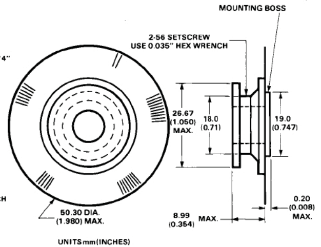
Figure 5. HEDS-6100 Codewheel.
