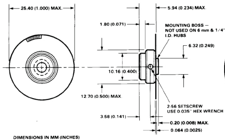
Figure 5. HEDS-6100 Codewheel.
